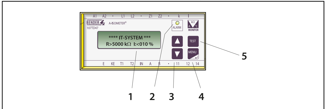
Fig. 1: Operating elements
