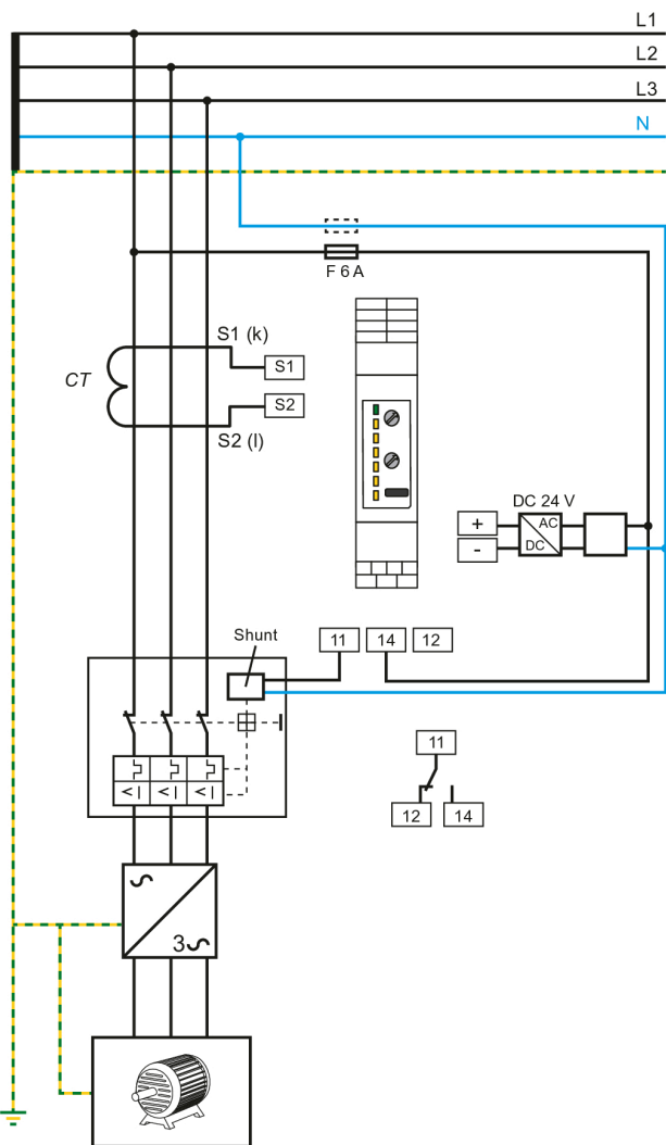
Wiring diagram with shunt release
